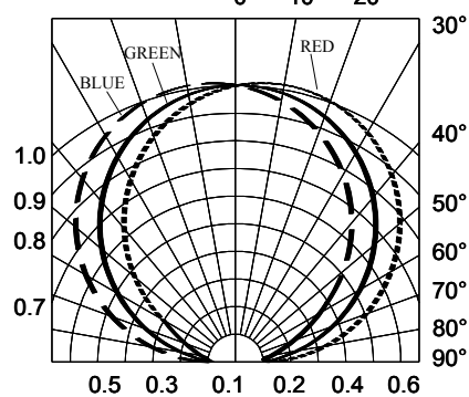
Radiation Diagram
