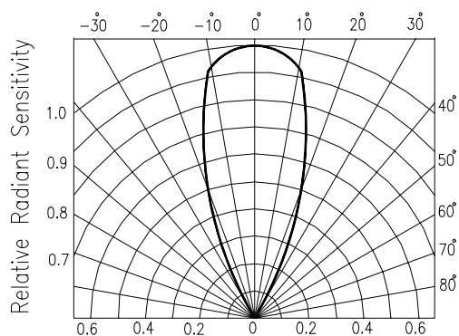
Fig. 7 Relative Radiant Sensitivity vs. Angular Displacement
